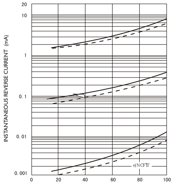
FIG.4-TYPICAL REVERSE CHARACTERISTICS
